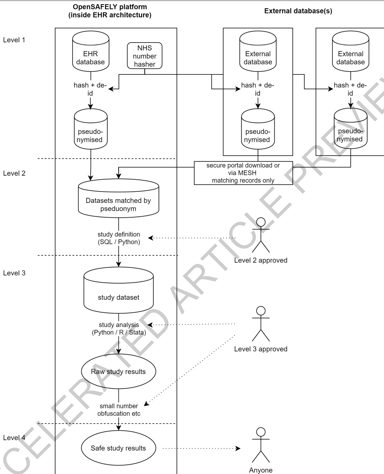
Extended Data Fig. 2 | Illustration of data flows in the OpenSAFELY platform.
